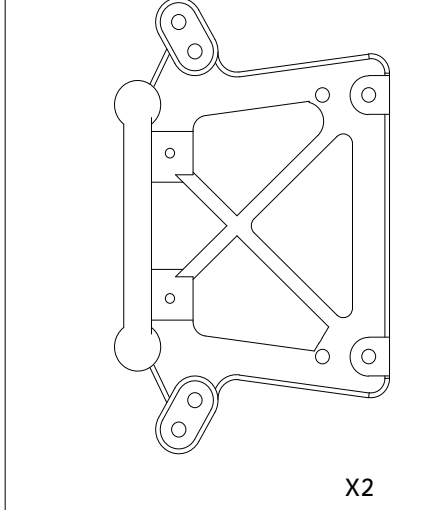
205058 Skid Plate Bumper Set / Unterbodenschutz
